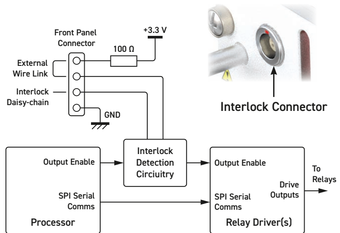
Interlock Signal Routing Diagram for 65-233
